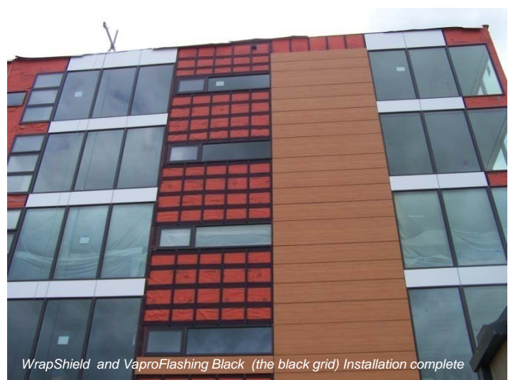
Detail of WrapShield with VaproFlashing Black under open joint cladding
