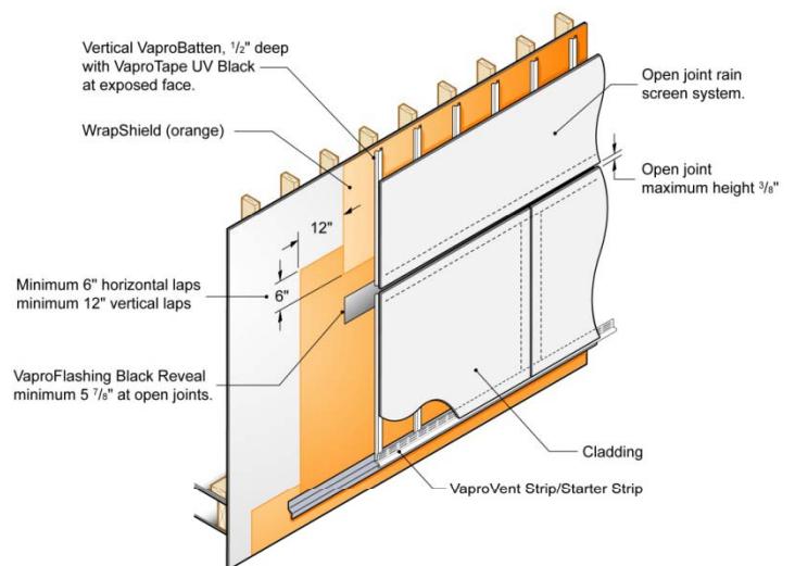
Detail of WrapShield with VaproFlashing Black under open joint cladding
