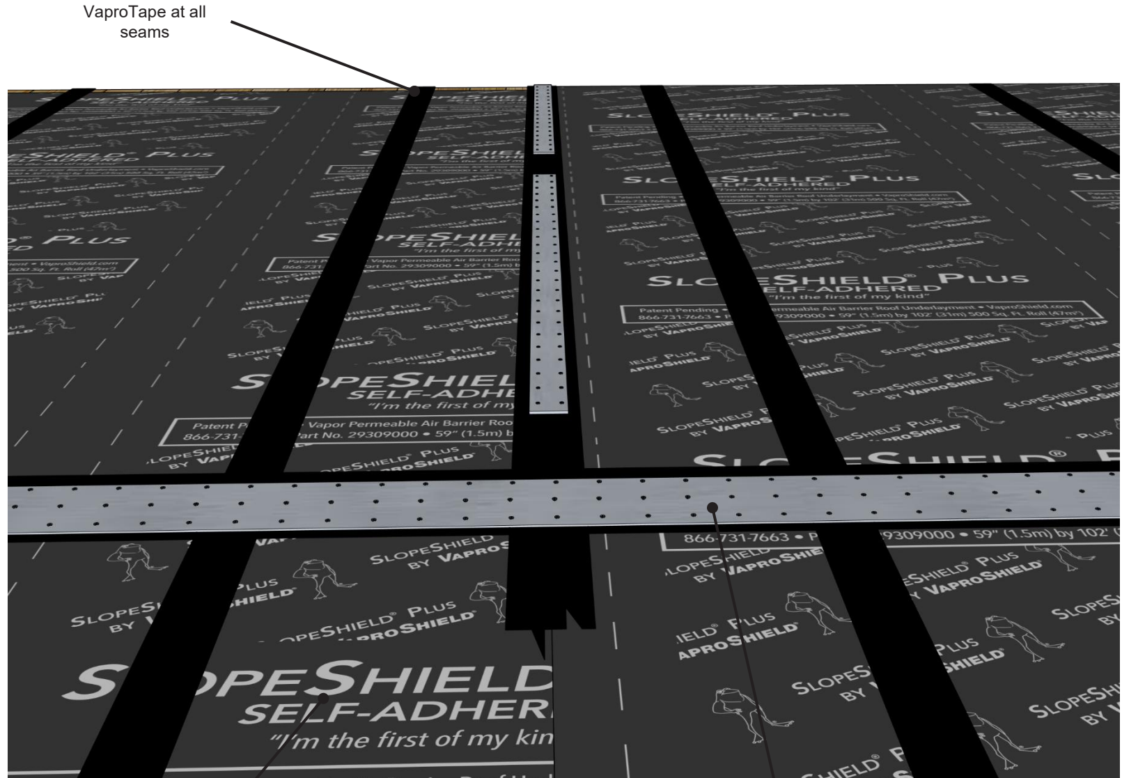
SlopeShield Plus SA installed over mass timber
